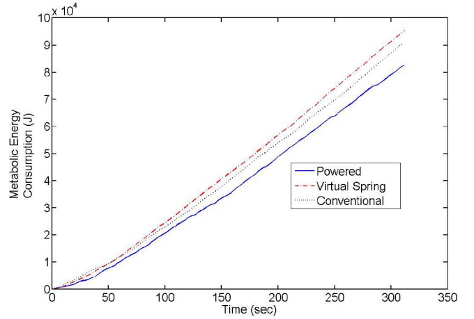
Fig. 18. Metabolic energy consumption of amputee participant 1 walking at a self-selected speed for three conditions: 1) using their conventional passive prostheses (conventional); 2) using the powered prosthesis with only a virtual spring response (virtual spring); and 3) using the powered prosthesis with a nonconservative, motive power output (powered).
